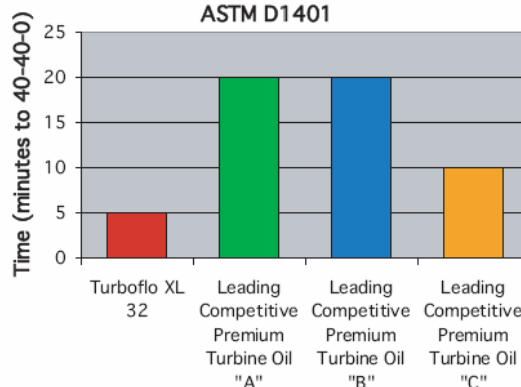
Mechanical Emulsion Test ASTM D1401
